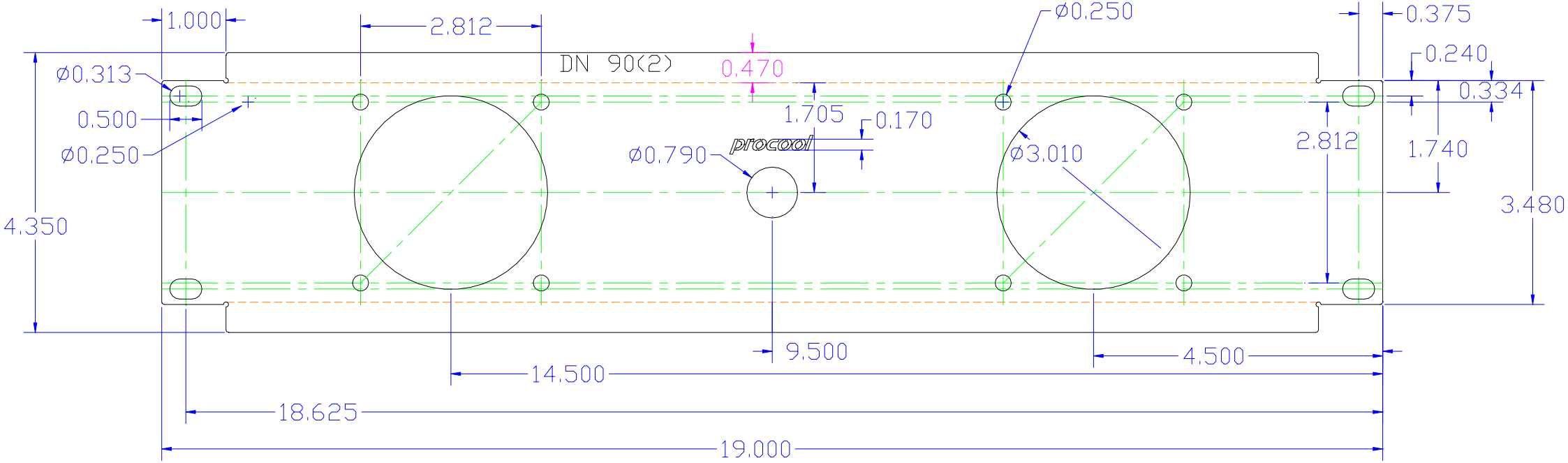
RACK FANS PROCool 2U-2X TWO FANS CENTER SWITCH
